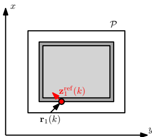
Subgrid \mathcal{P} around the obstacle
