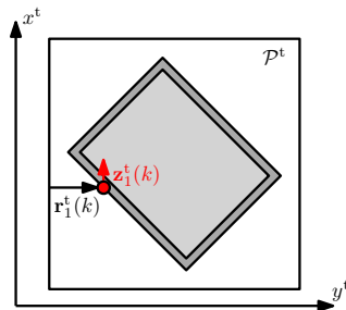
Rotated subgrid \mathcal{P}^t
