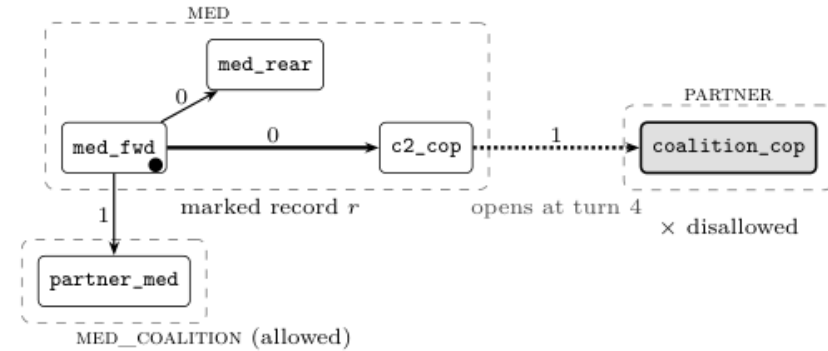
(a) informational sort: runtime topology
