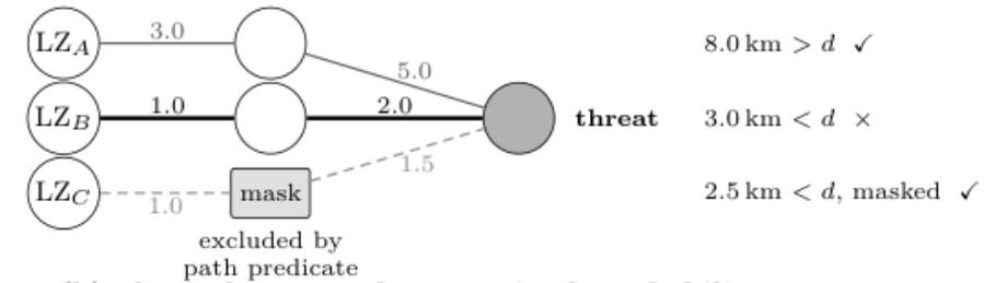
(b) physical sort: path-constrained reachability
